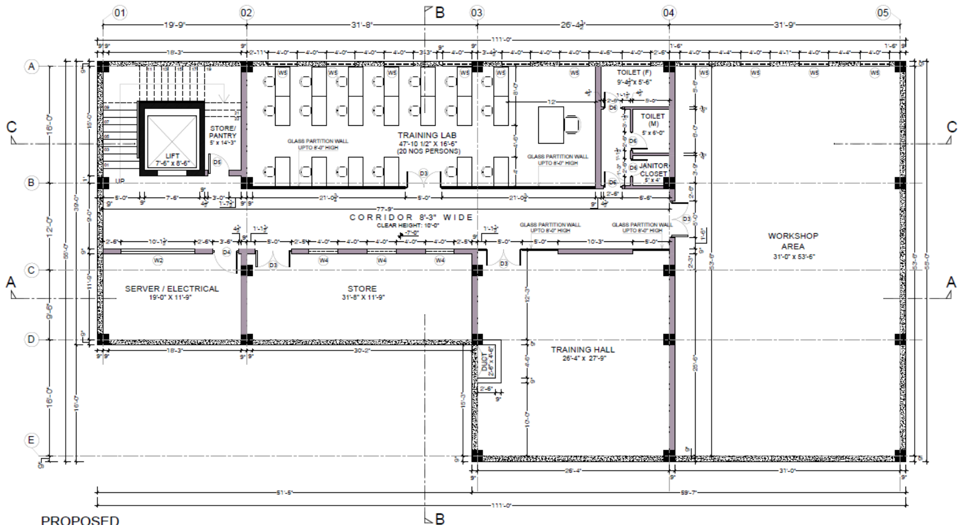
PROPOSED LOWER GROUND FLOOR PLAN COVERED AREA = 5270 Sft
