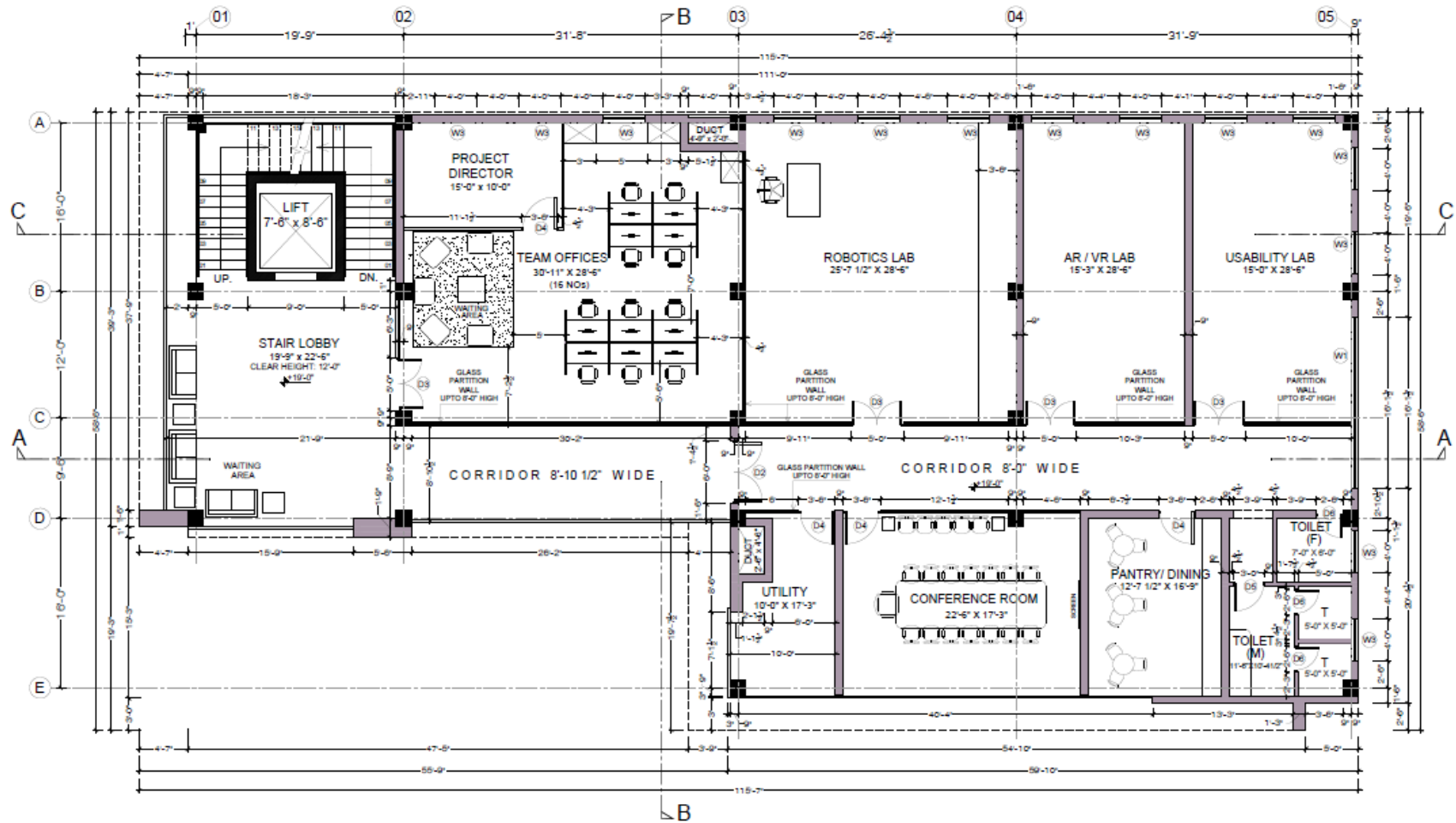
PROPOSED FIRST FLOOR PLAN COVERED AREA = 5890 Sft
